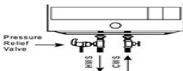
Fig. 6 - Pressure Relief Valve
