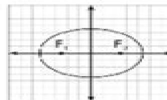
Ellipse
