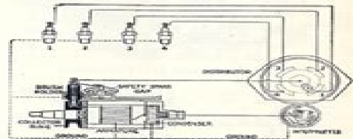
Circuit Diagram Type DU-4 Magneto
