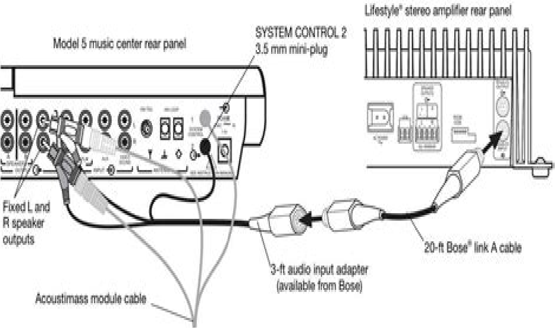
Figure 14 Lifestyle® stereo amplifier to Model 5 music center connections
