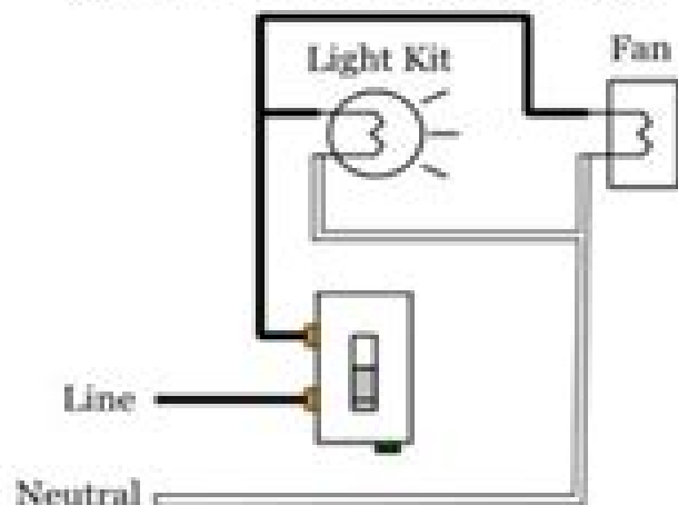
One wire/switch configuration
