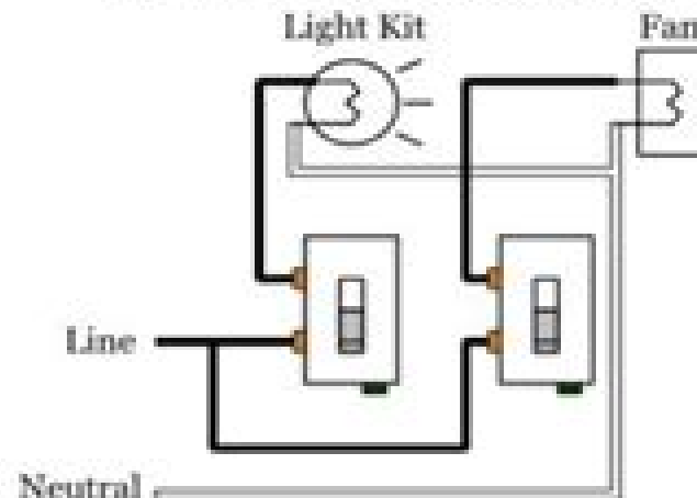
Two wire/switch configuration
