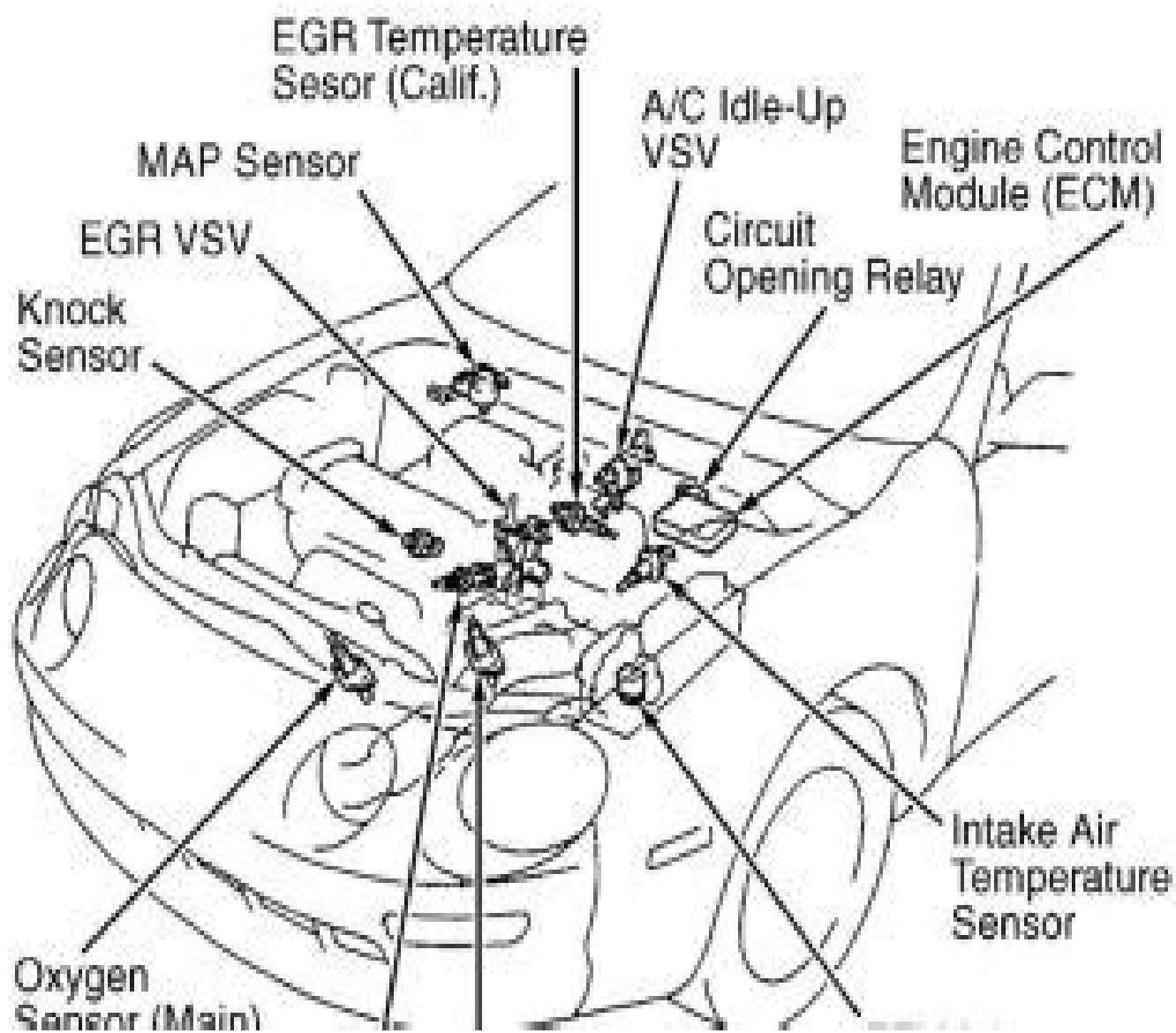
1994 Toyota Celica GT Fig. 1: Component Locations (1 Of 4)
