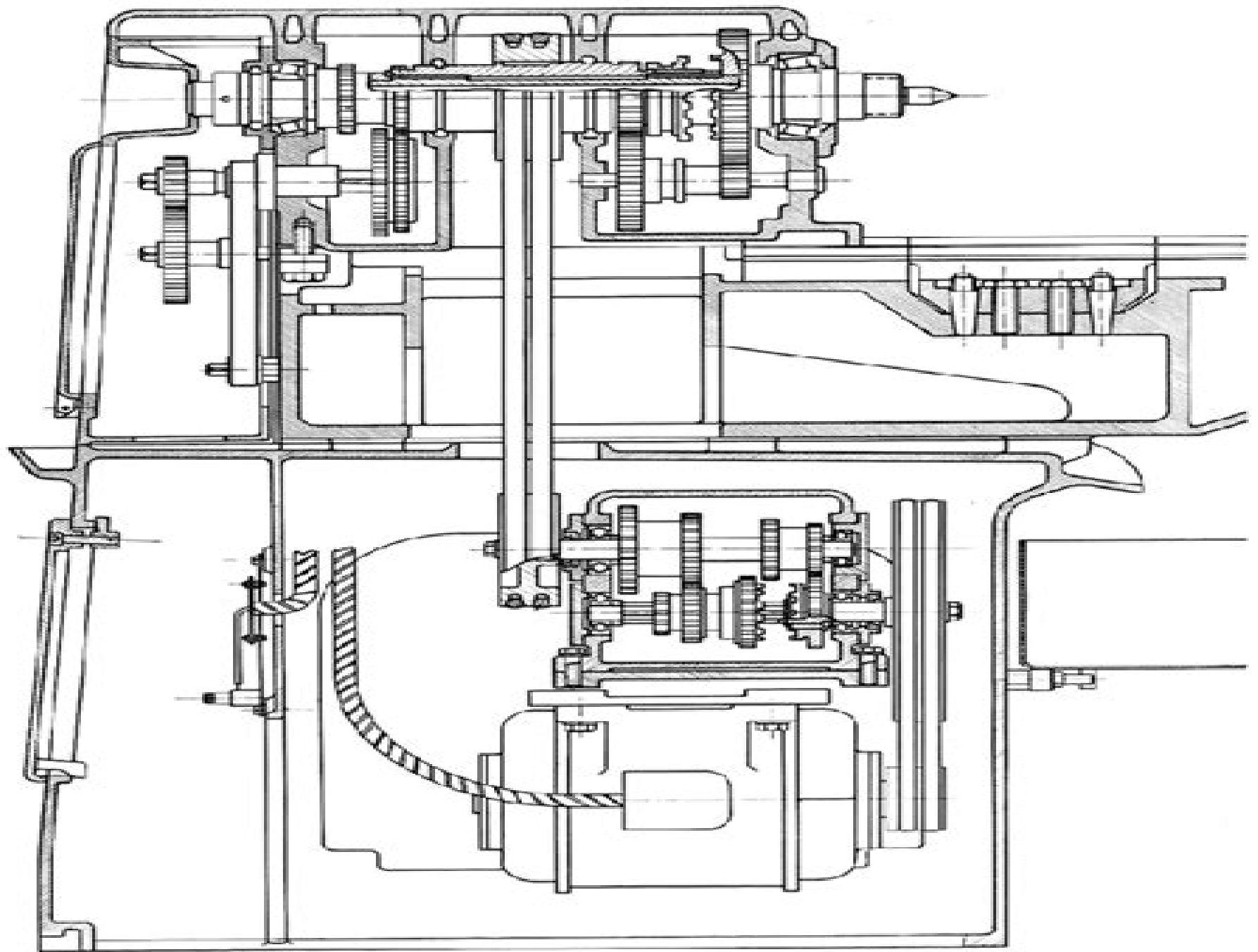
Celtic 14 lathe headstock internals with the slow-speed
