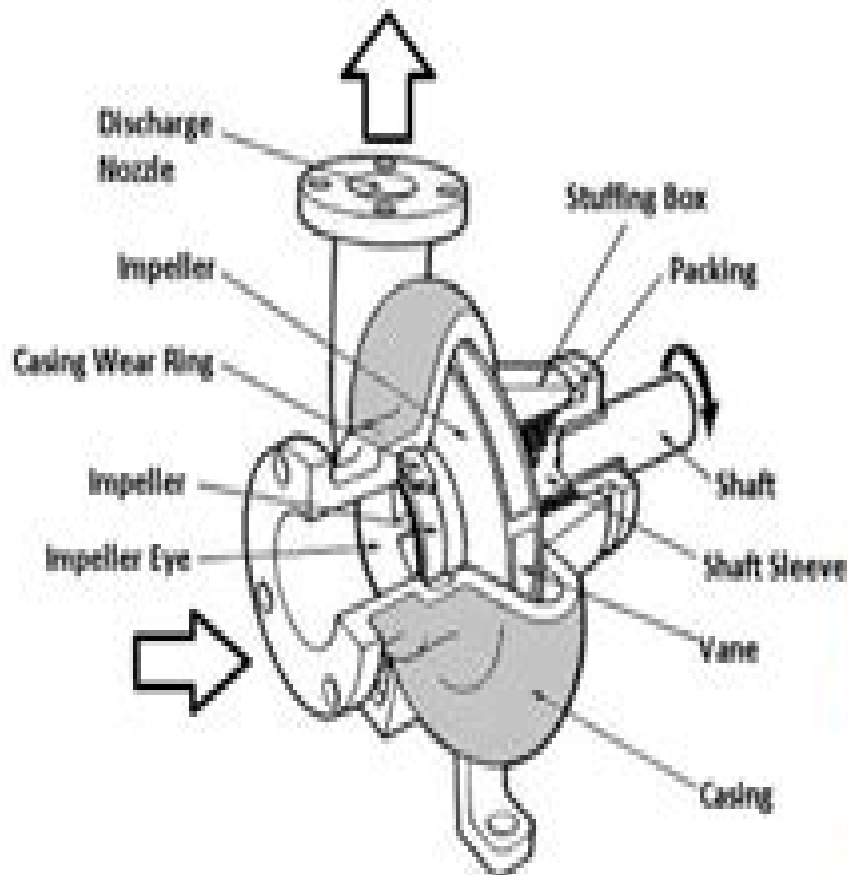
Parts of Centrifugal Pump
