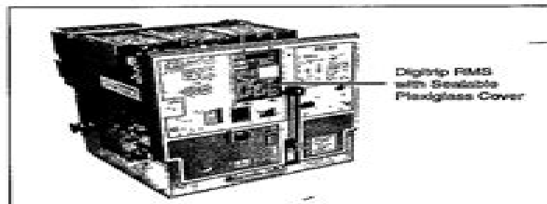
Figure 1 DSII-620 Circuit Breaker with Digitrip RMS Trip Unit Installed
