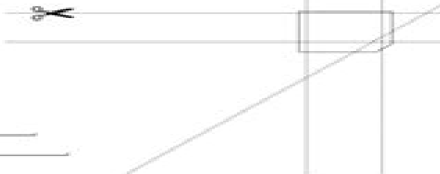
MicroSIM (3FF) to NanoSIM (4FF)
