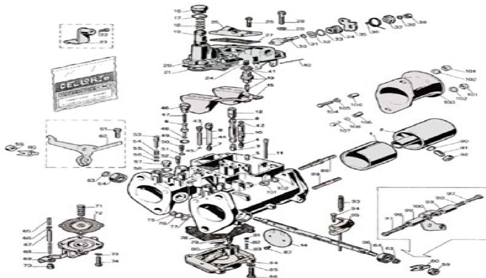
DELLORTO 45 DHLA M - exploded view
