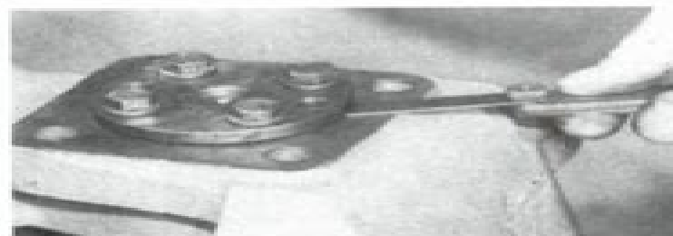
Fig. 9—To set bearing pin preload, use a feeler gage to measure gap between bearing pin flange and stub axle housing. Refer to text.
