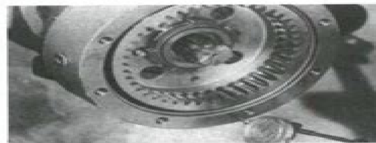
Fig. 10—To set stub axle bearing preload, mount a dial indicator so probe contacts face of wheel hub. Measure and play and refer to text.
