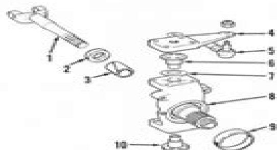
Fig. 9—Exploded view of David Brown front drive stub axle showing component parts and their relative positions.
