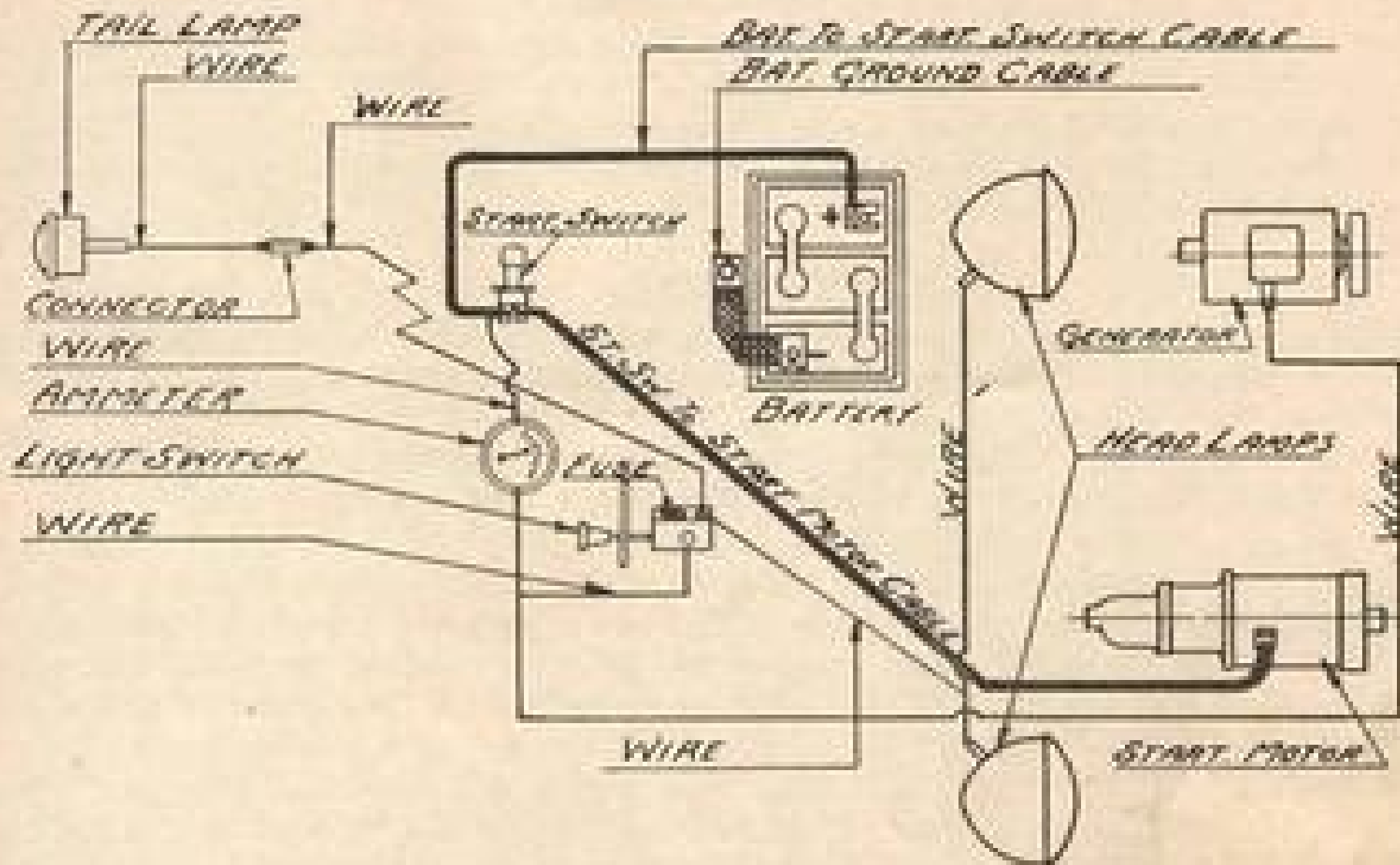
Fig. 31. Wiring Diagram of Electrical System
