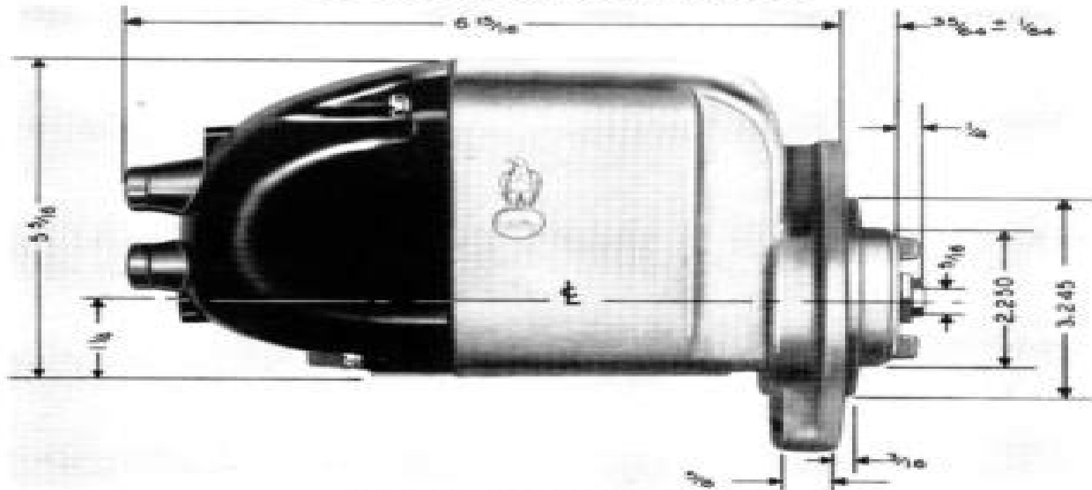
Figure 2. Model 41 Magneto Dimensions
