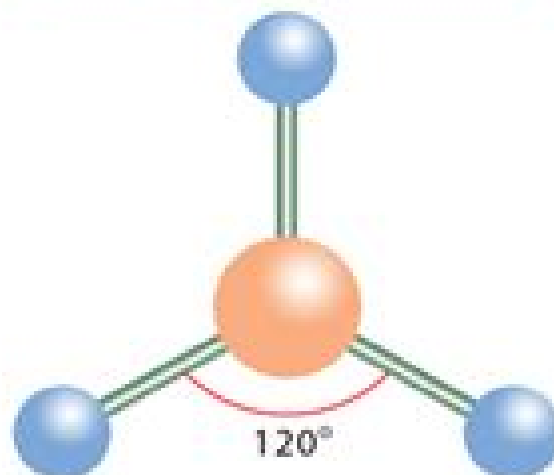
Trigonal Planar
