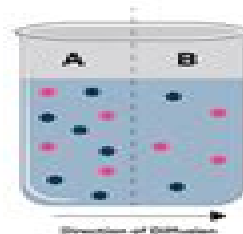
Figure 2: Molecules diffuse down concentration gradients to achieve equilibrium. Select the image to enlarge.
