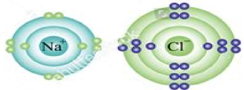
Ionic Bonding
