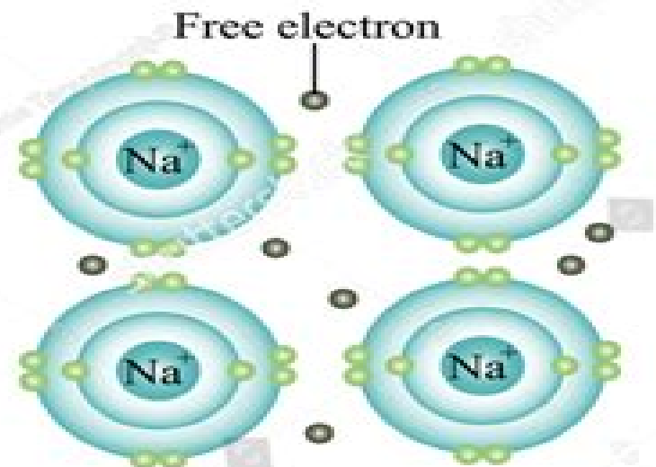
Metallic Bonding
