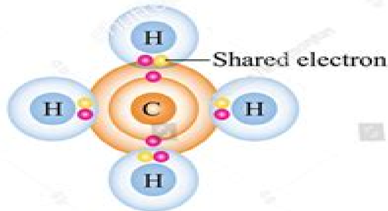
Covalent Bonding
