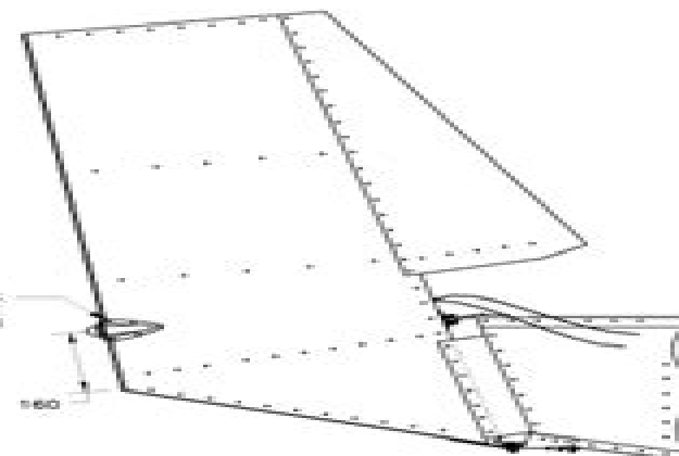
POSITION LIGHT DRILL/CUT OR FILE A 1" HOLE IN THE FIBERGLASS MOUNTING BRACKET FOR THE LIGHT FIXTURE BODY.
