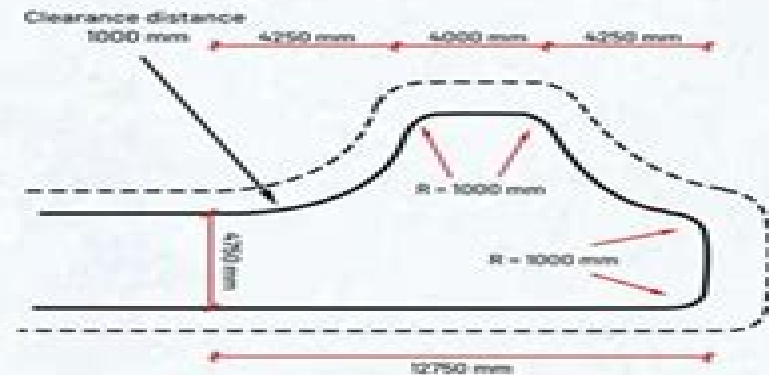
Hammerhead turning place for cars
