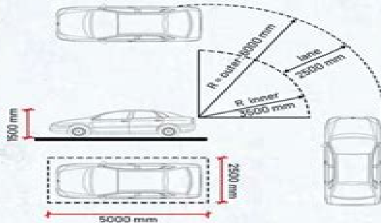
Comfortable turning radius for a car
