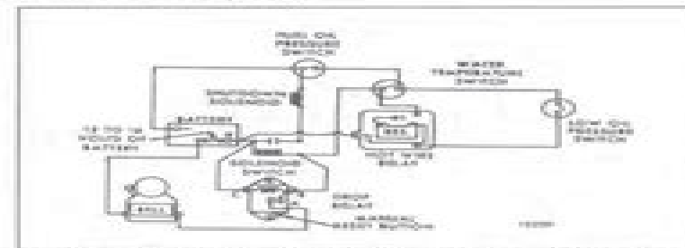
Fig. 3 - Alarm Bell Connected to Electrical Shutdown System
