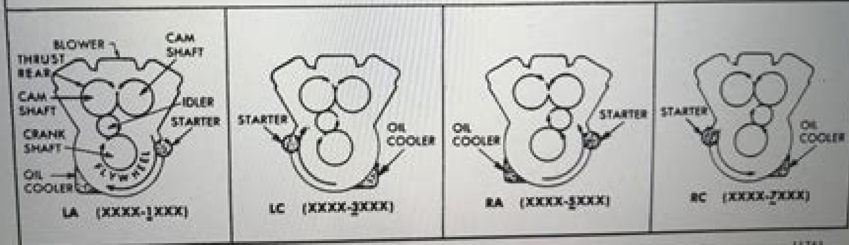
Fig. 3 - V-Type Engine Model Description, Rotation and Accessory Arrangement
