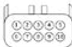
ENGINE HARNESS SIDE
