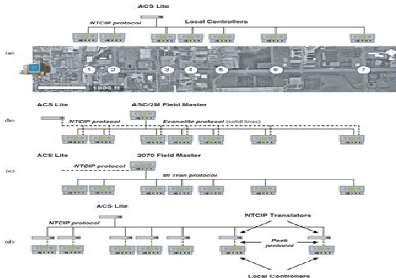
FIGURE A1 ACS Lite as deployed with (a) Siemens, (b) Econolite, (c) McGraw-Hill, and (d) Peek.
