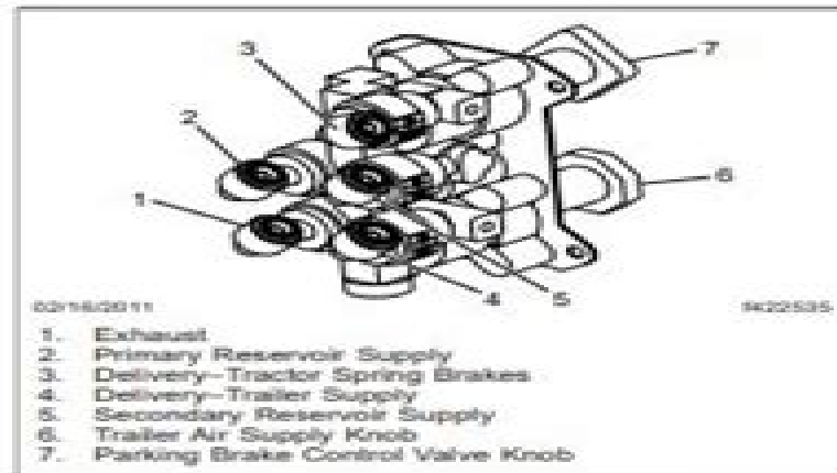
Fig. 1, MV-3 Parking Brake Valve
