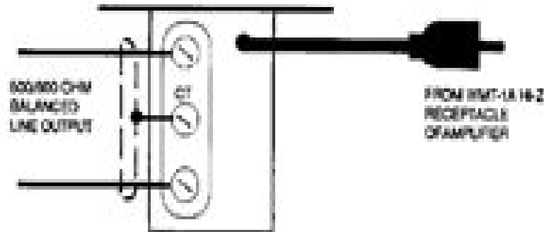
Figure 3 — Connecting WMT-1A as Output Matching Transformer
