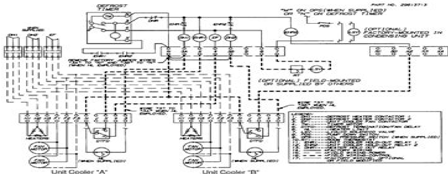
Diagram 10. Typical Wiring Diagram for Multiple Evaporators Defrost and Evaporator Fan Contactors with Unit Cooler Holdout Relay
