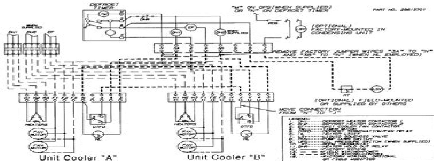
Diagram 9. Typical Wiring Diagram for Multiple Evaporators with Heater Limit Defrost and Evaporator Fan Contactors
