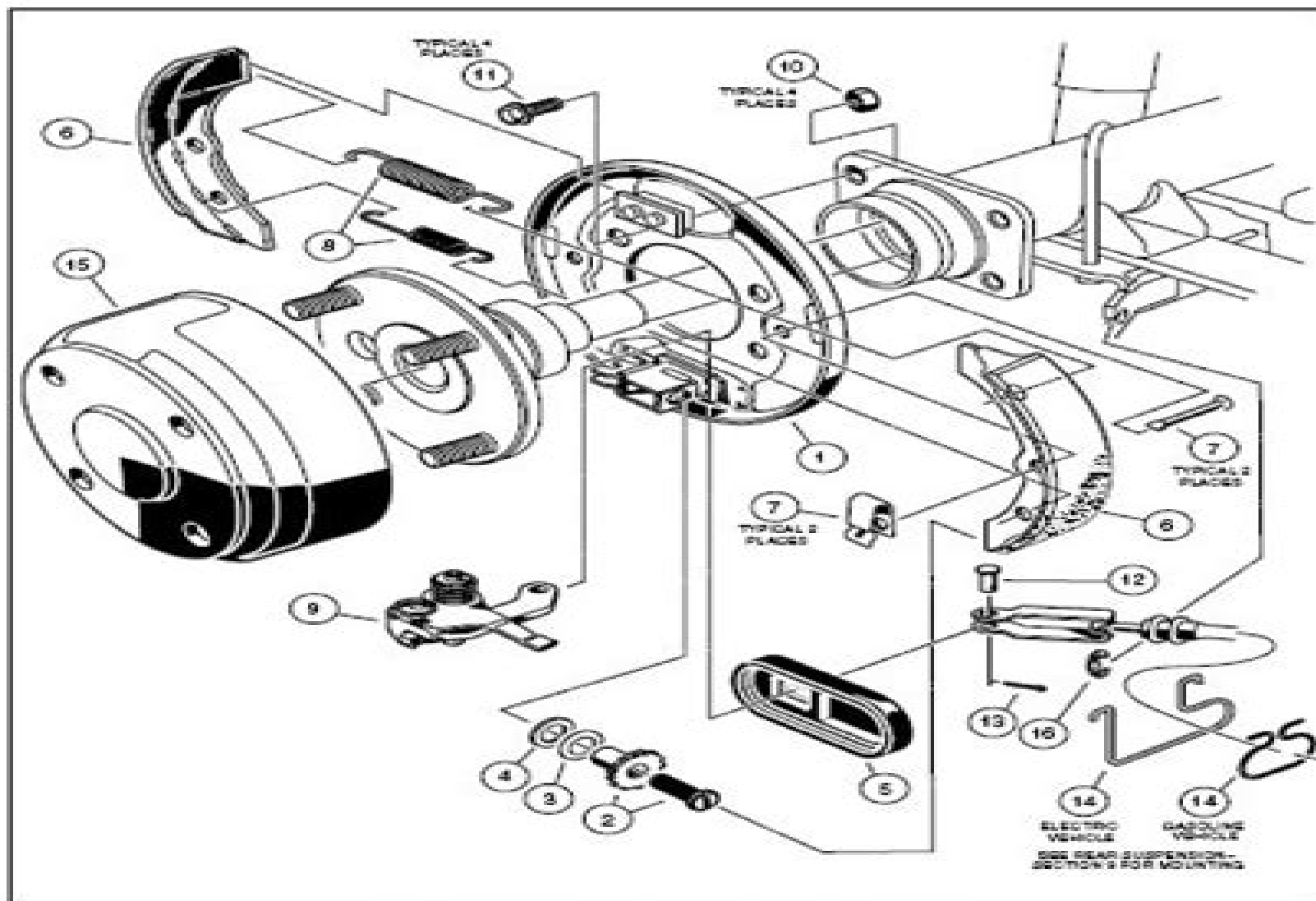
Figure 6-1 Self-adjusting Wheel Brake Assembly
