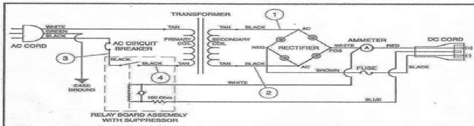
Figure 6-9 PowerDrive 3 Battery Charger Wiring Diagram (External Charger)
