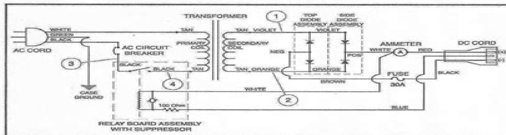
Figure 7-9 PowerDrive 3 Battery Charger Wiring Diagram (External Charger)
