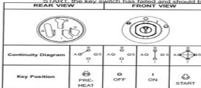
Figure 12-12 Key Switch Terminals and Continuity Diagram
