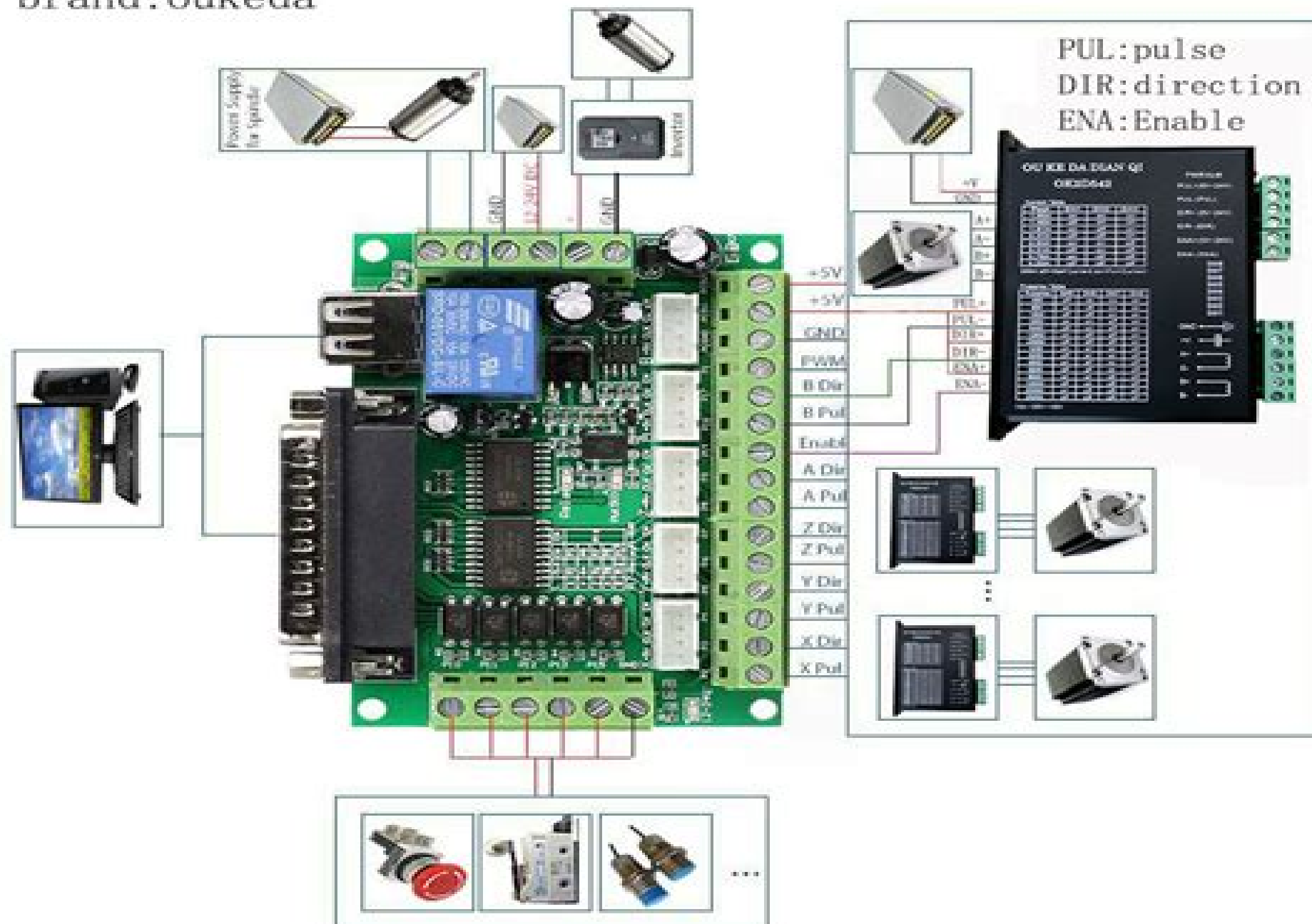
5 Axis CNC Breakout Board Interface Mach3 CNC Router Kit
