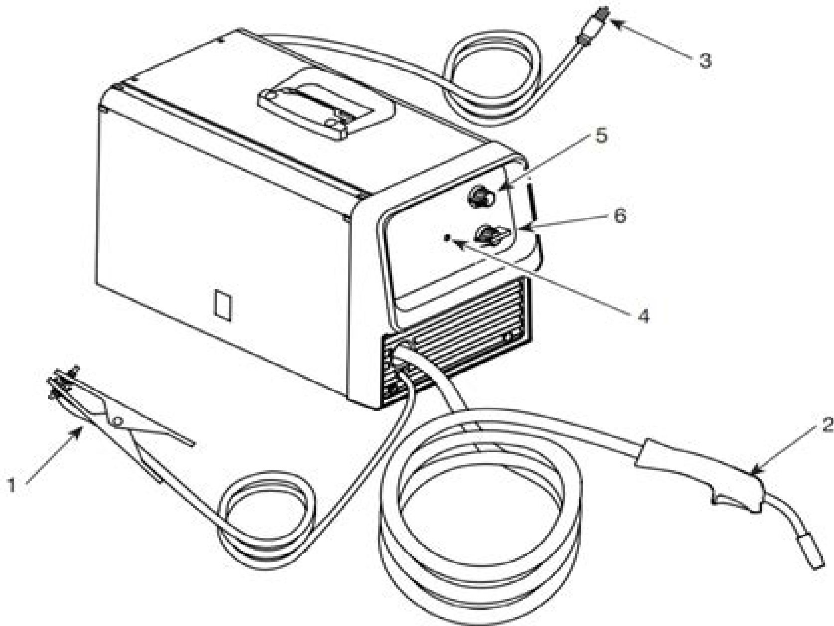
Figure 1 - Welder Components and Controls
