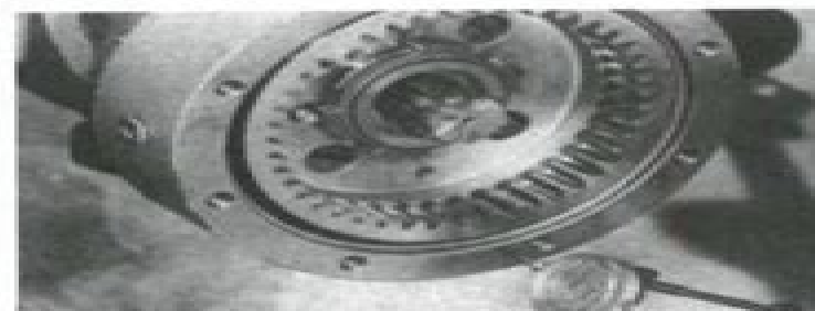
Fig. 10—To set stub axle bearing preload, mount a dial indicator so probe contacts face of wheel hub. Measure end play and refer to text.
