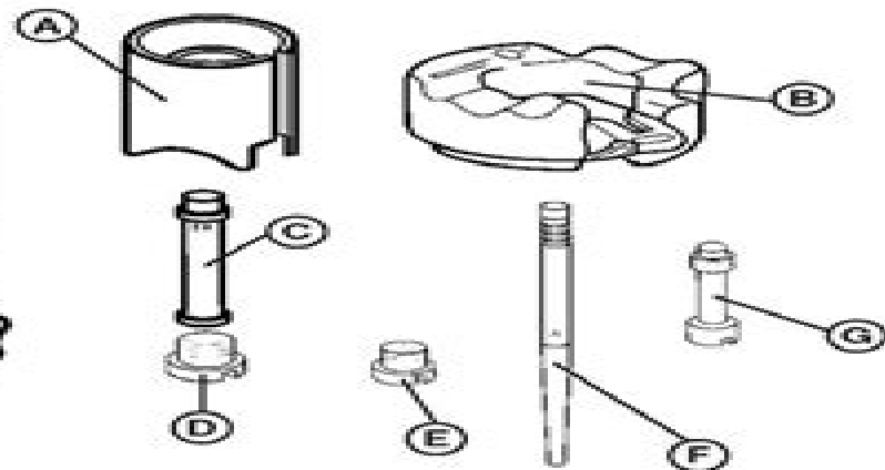
The basic calibration elements of a carburetor. A: Throttle valve; B: Float; C: Atomizer; D: Main jet; E: Idle jet; F: Tapered Needle; G: Starter jet.
