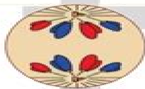
Anaphase
