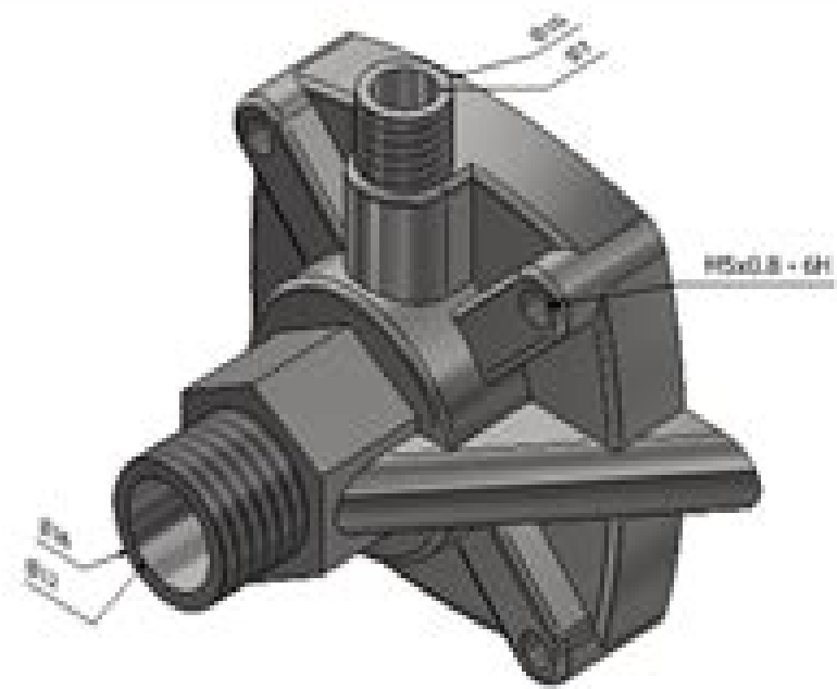
ISO VIEW ( 2 : 1 )
