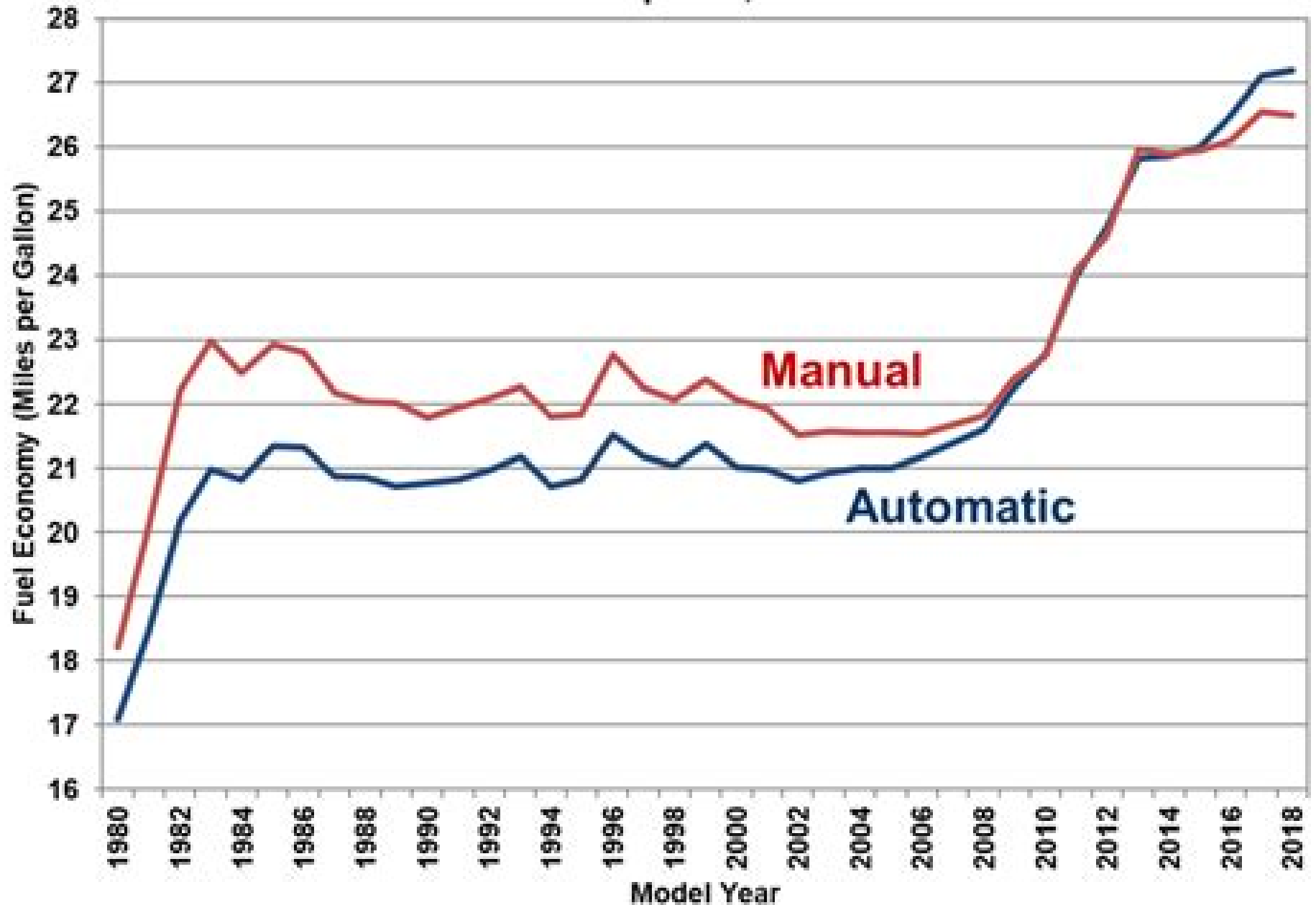
Fuel Economy for Vehicles which have both Manual and Automatic Transmission Options, Model Years 1980-2018
