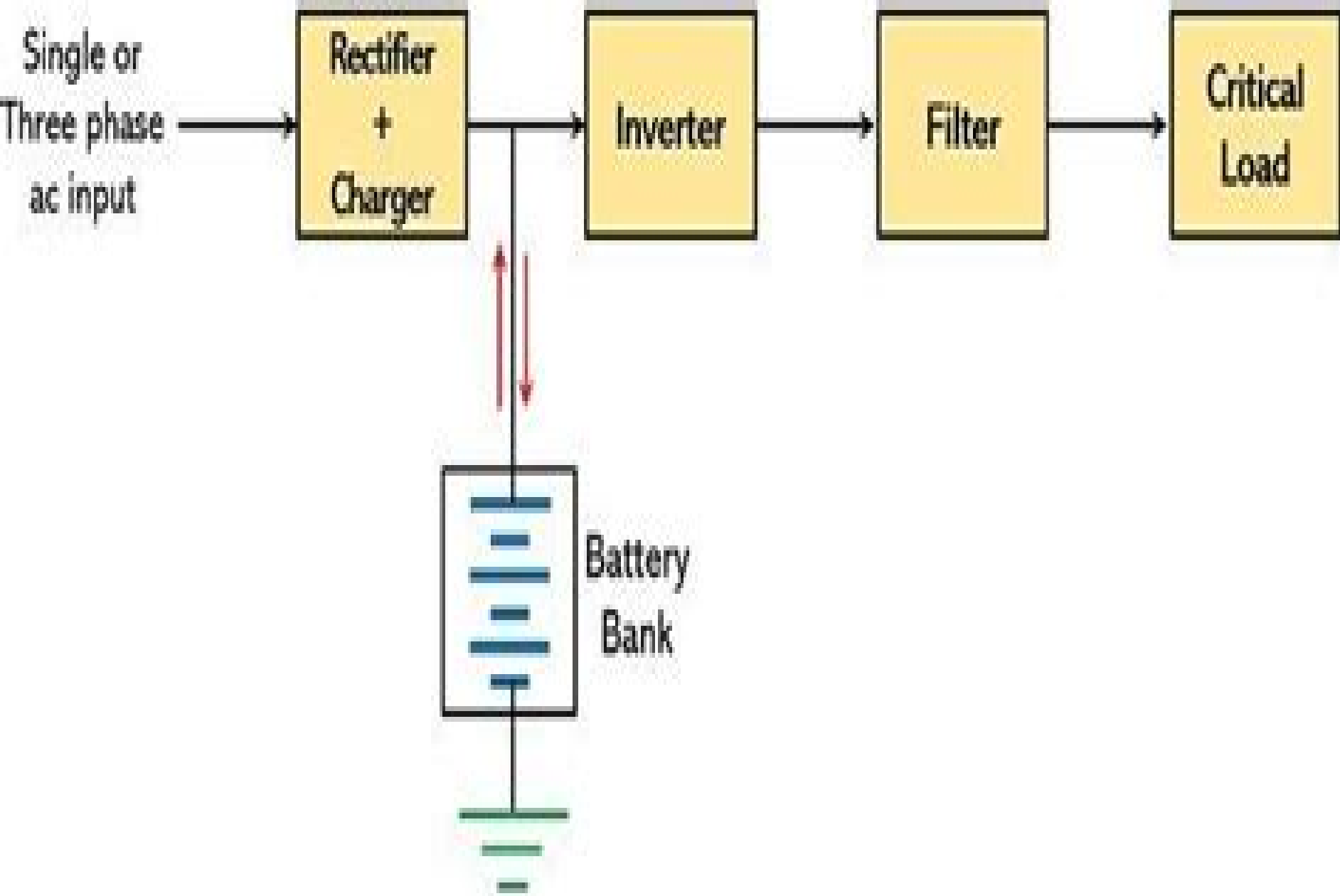
Block Diagram of typical UPS System
