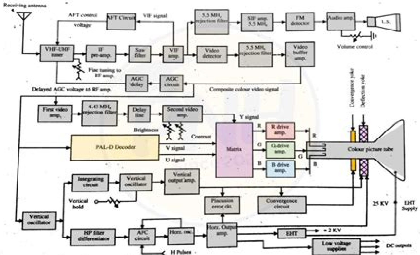
Block Diagram of PAL-D Color TV Receiver
