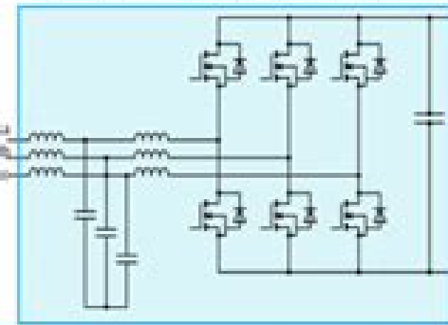
Voltage Source Converter (AC to DC)
