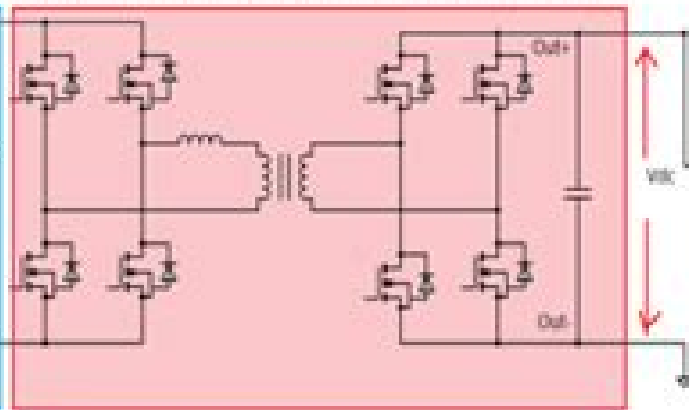
Dual Active Bridge Converter (Medium DC - Low DC)
