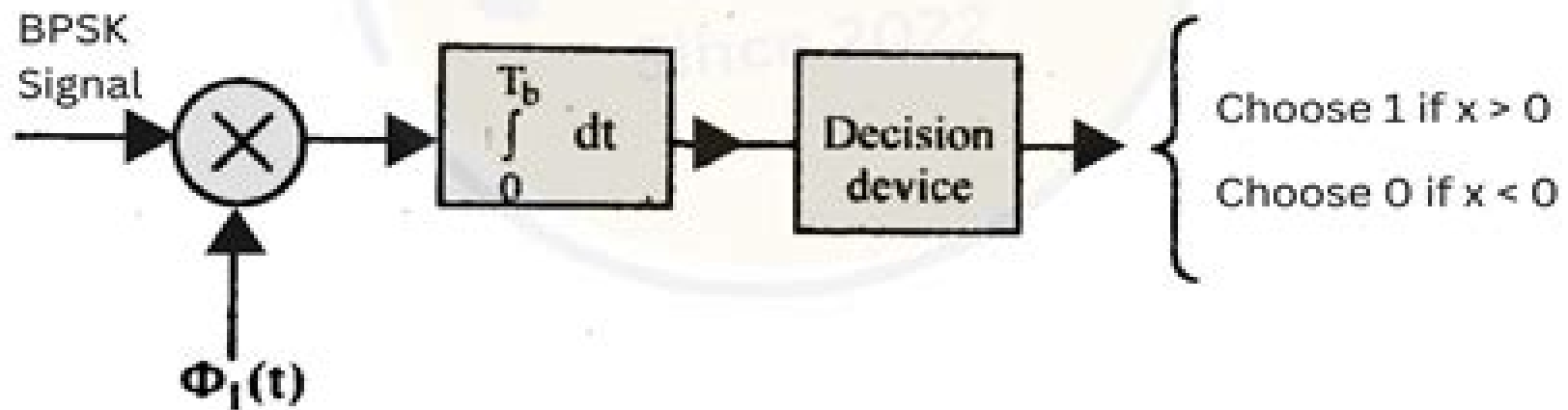
Block Diagram of BPSK Receiver
