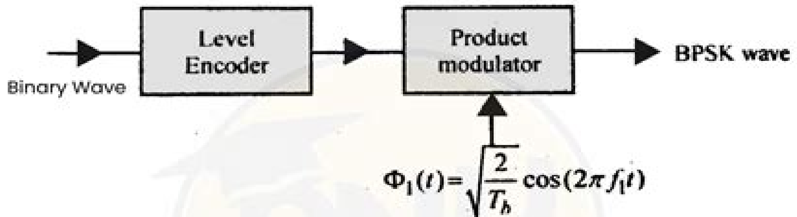
Block Diagram of BPSK Transmitter
