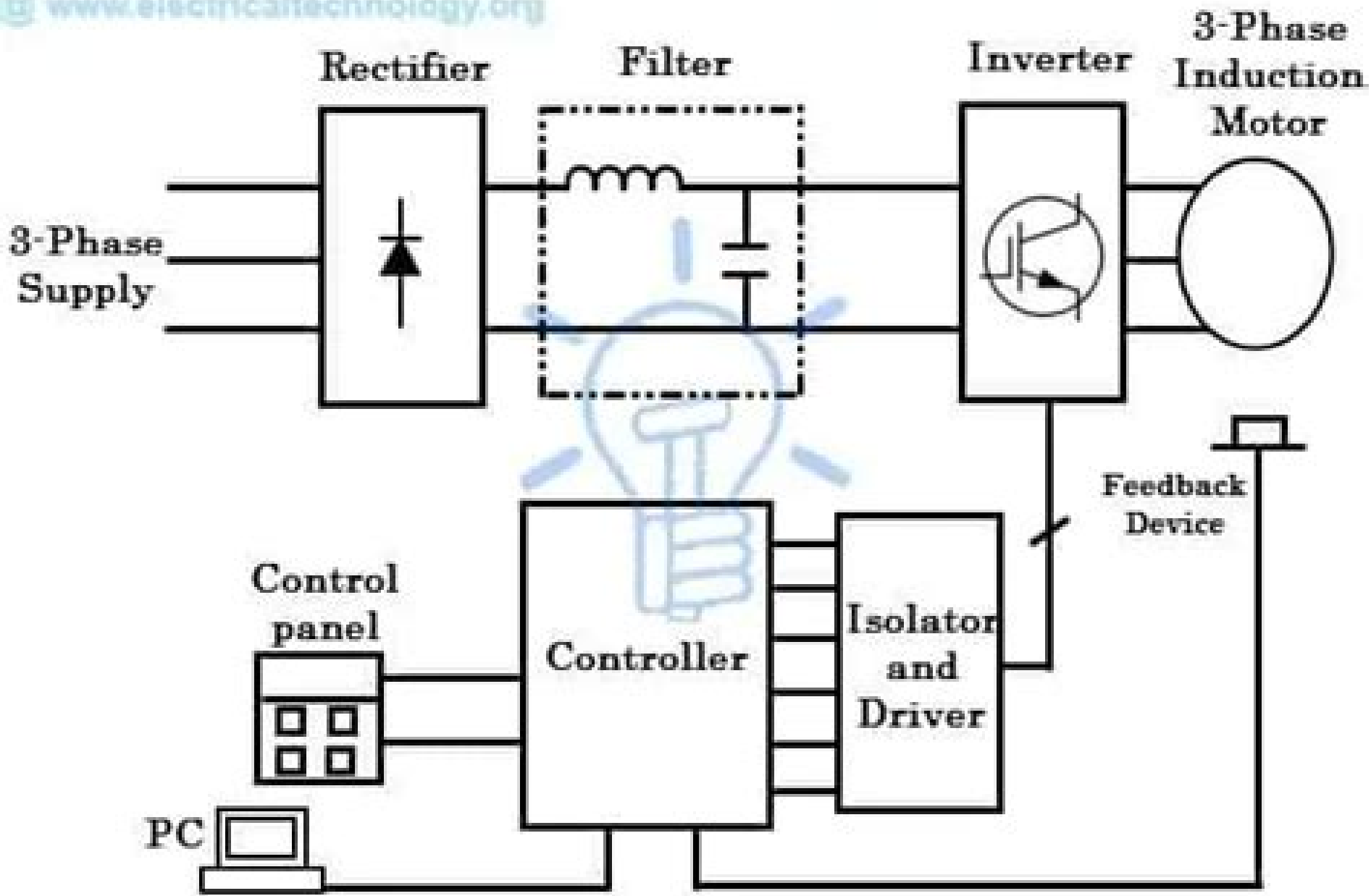
BLOCK DIAGRAM OF TYPICAL VFD (AC DRIVE)
