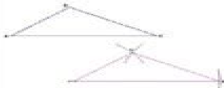
Triangle congruent to another
