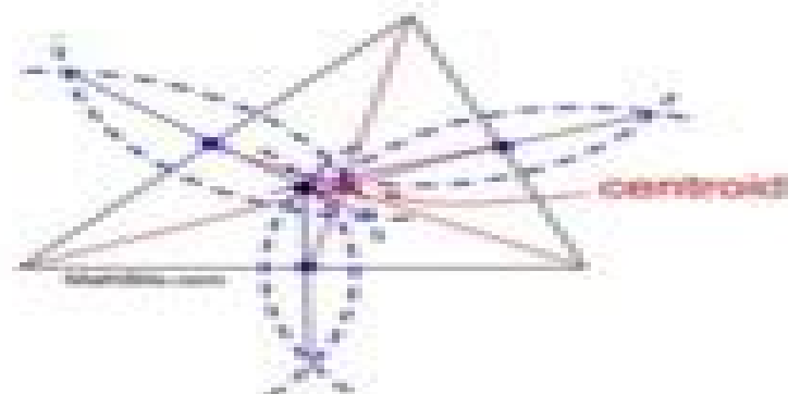
Centroid of a triangle 3-medians
