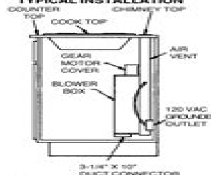
TYPICAL INSTALLATION
