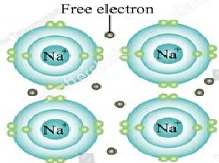
Metallic Bonding
