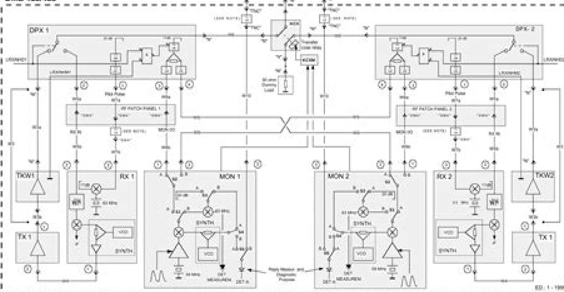
Figure 1.11. DME 415/435 - Main RF path signals - General simplified block diagram
