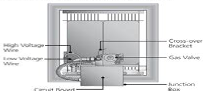
Figure 4.3 - Heater Components (rear view)
