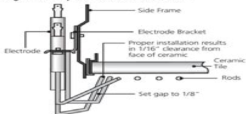
Figure 4.2 - Spark Electrode Side View
