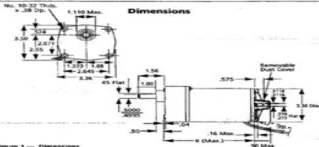
Figure 1 — Dimensions
