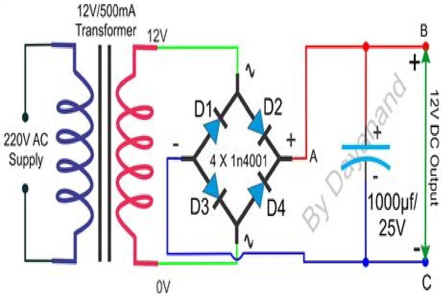
220V AC to 12V DC Converter
