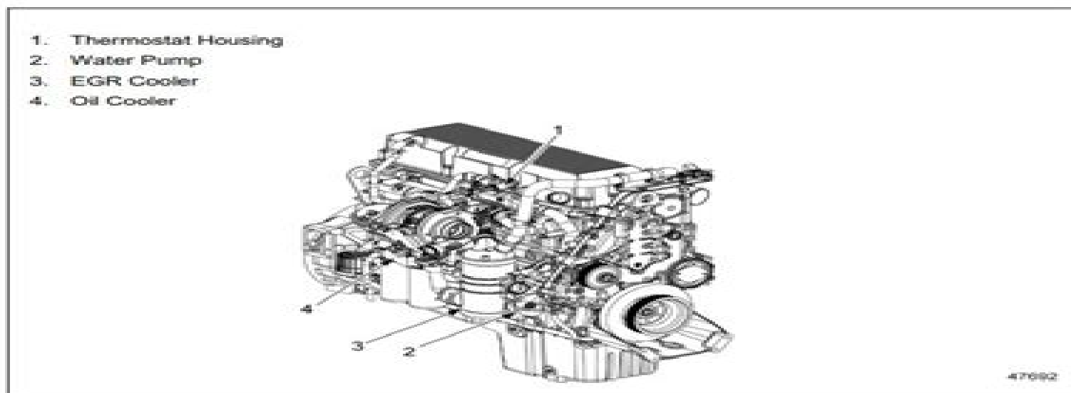
Fig 6.1, Cooling System Components
