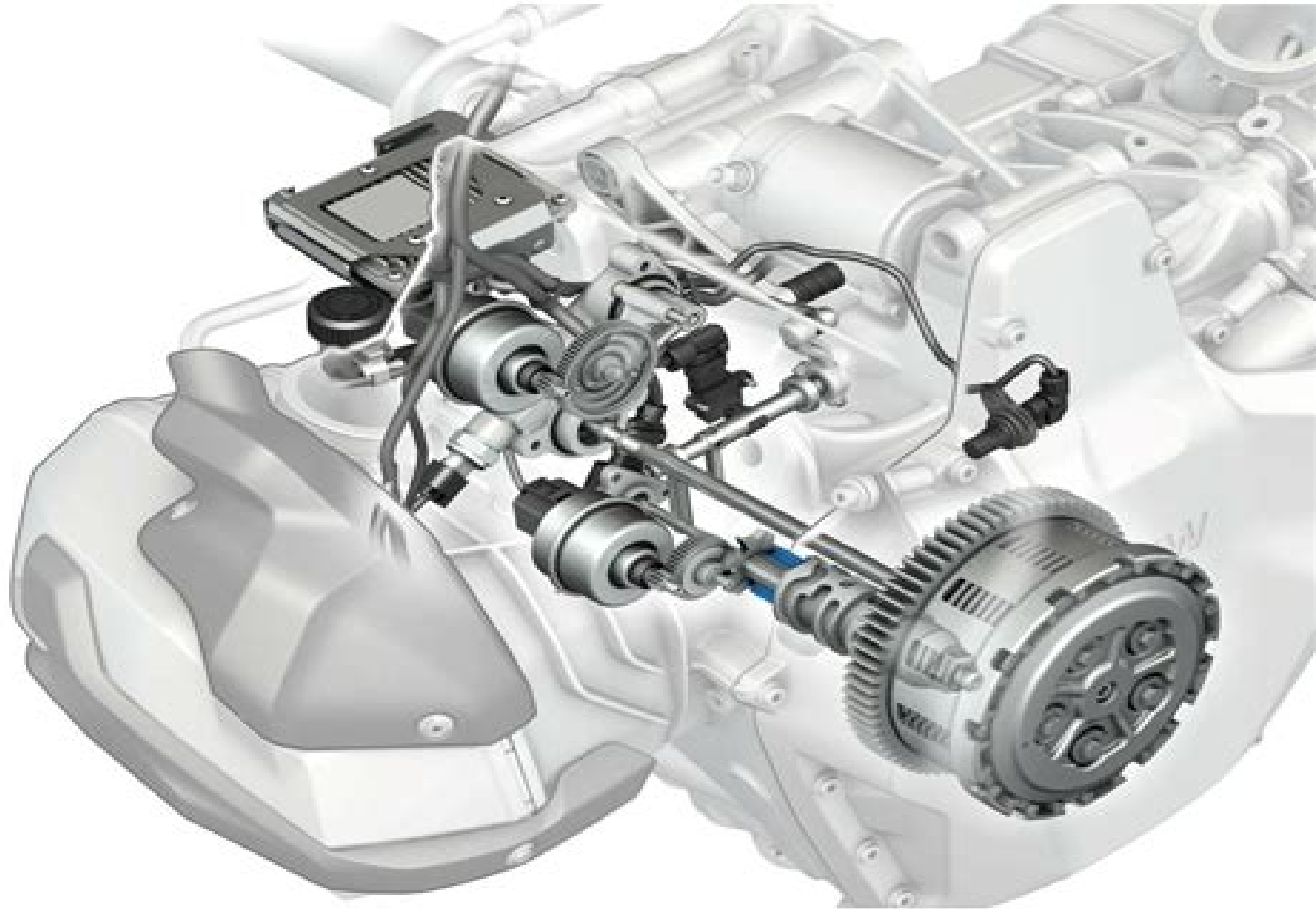
A schematic showing the new BMW Automated Shift Assistant (ASA) components in a Boxer engine/transmission. Image courtesy BMW
